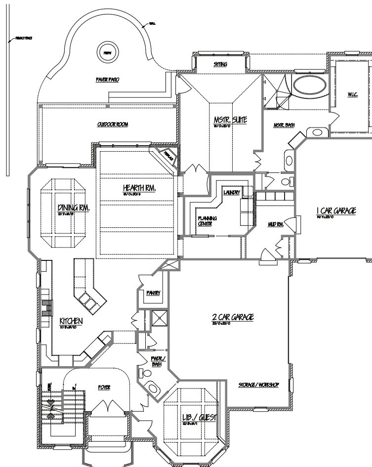
MAIN FLOOR 2,468 SQ. FT.
